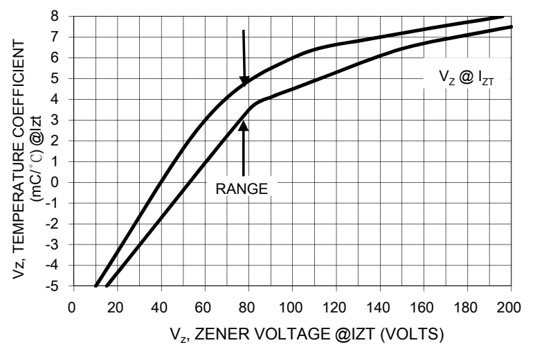
FIG.5 UNIT 13 - 200 VOLTS
